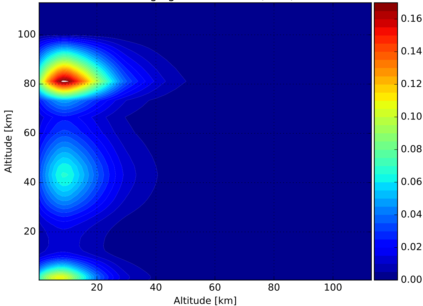
Averaging Kernel Matrix (VMR)
