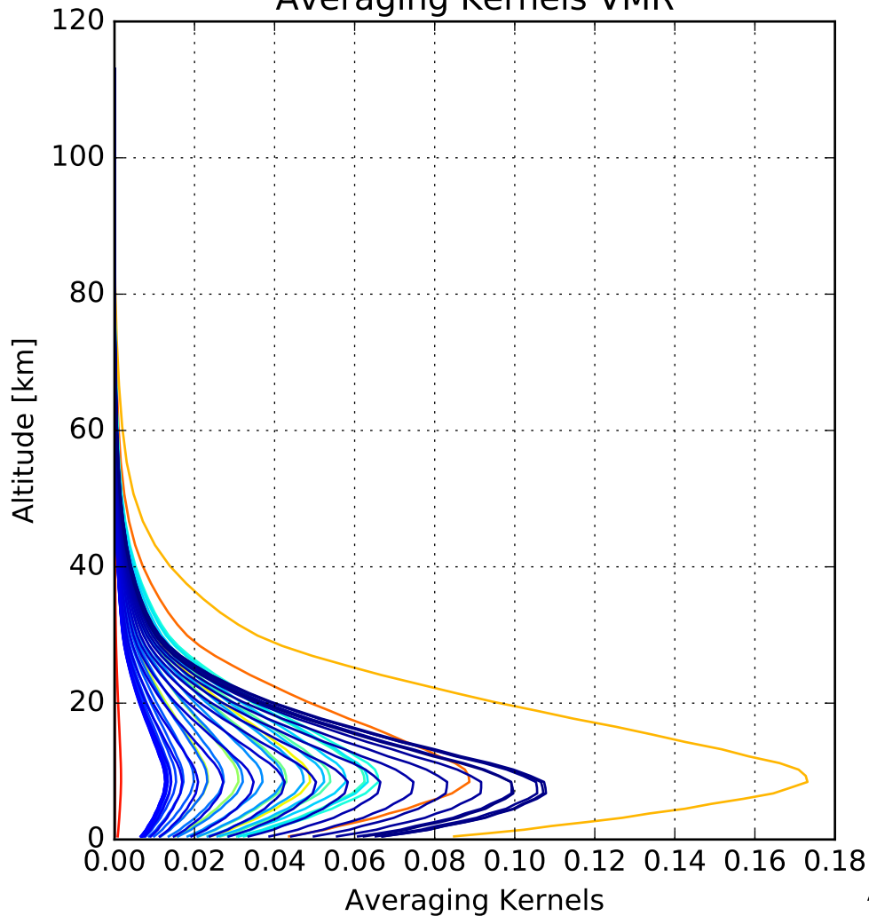
Averaging Kernels VMR
