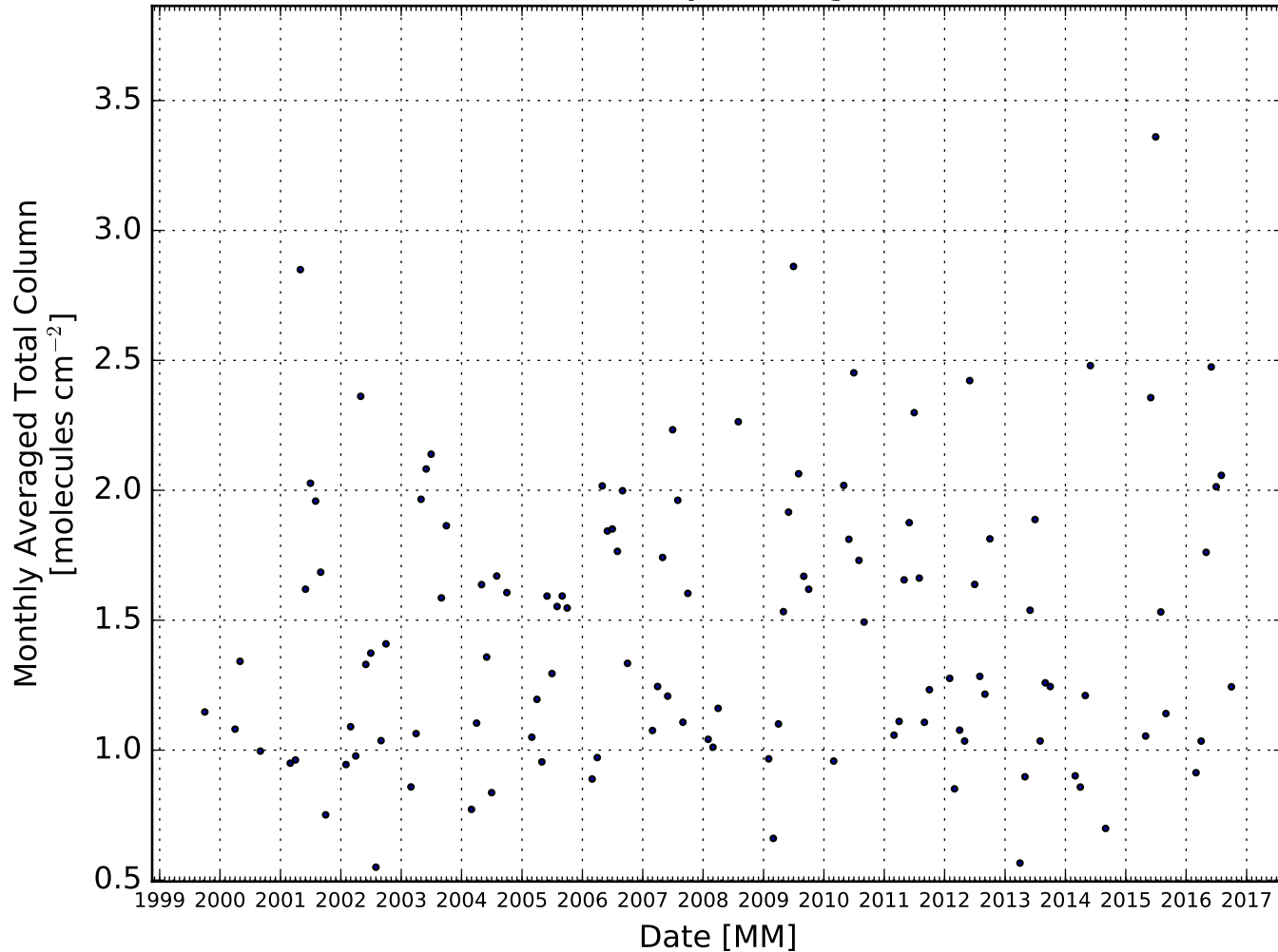
Time Series of Monthly Averaged Total Column
