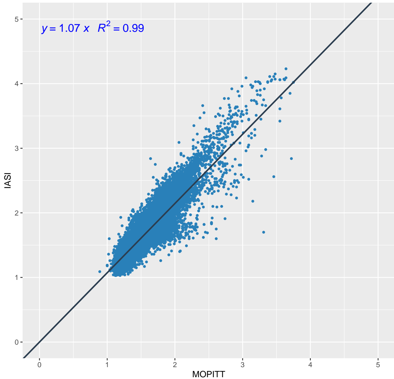
MOPITT IASI over water (September)
