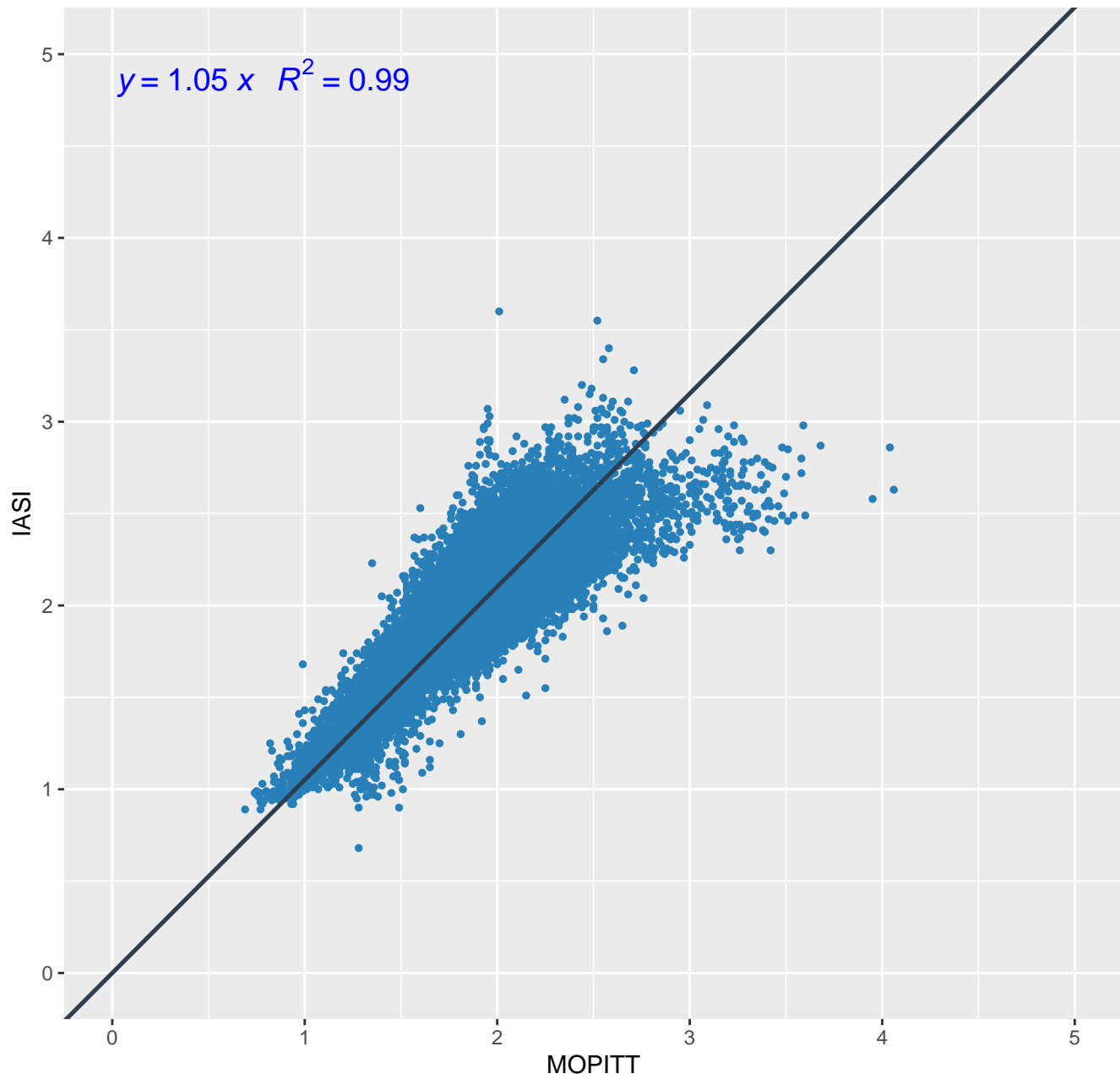
MOPITT IASI over land (May)
