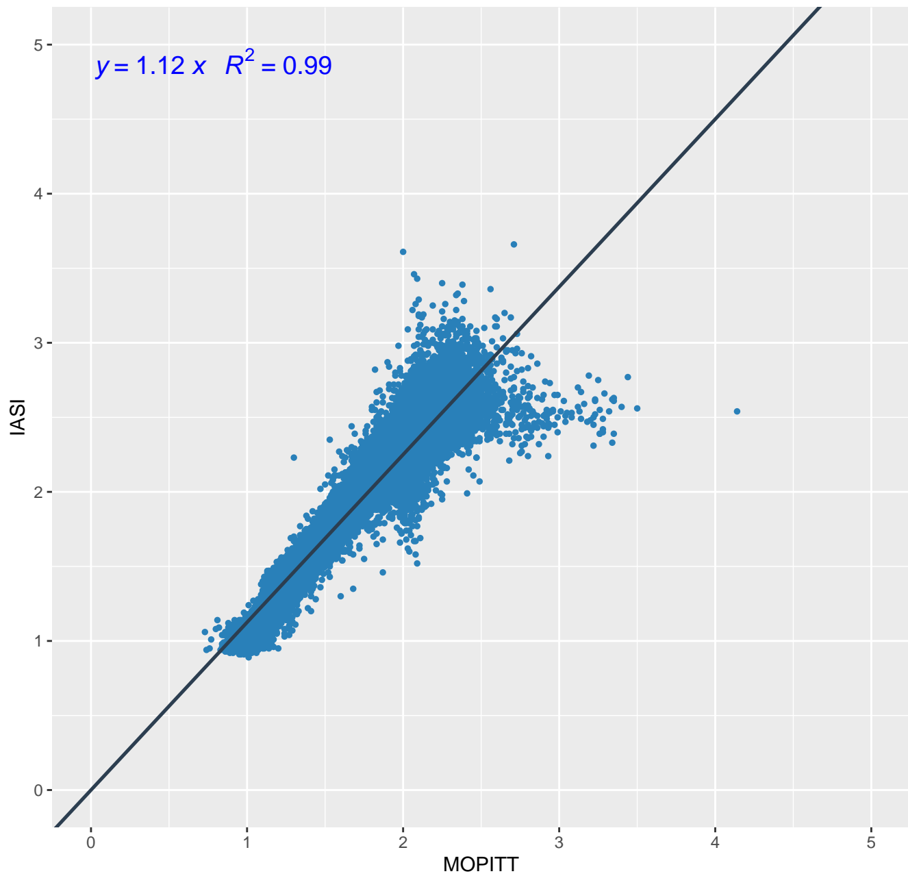
MOPITT IASI over water (May)
