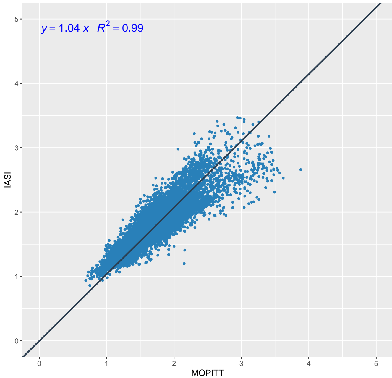
MOPITT IASI over land (June)
