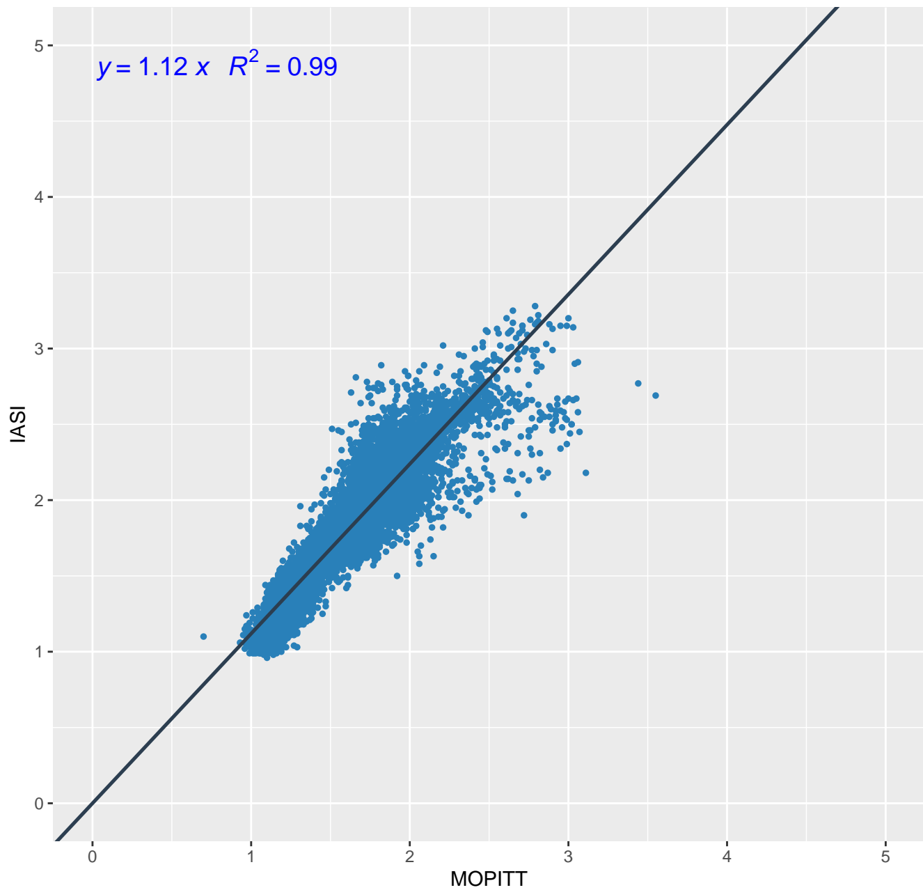
MOPITT IASI over water (June)
