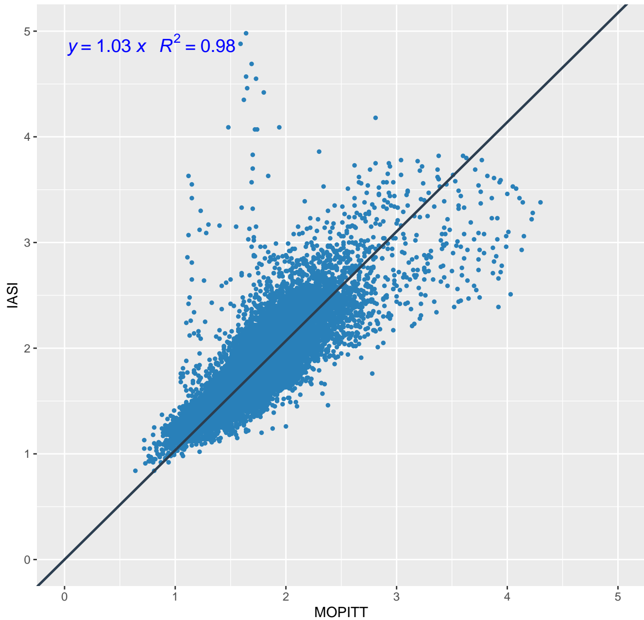
MOPITT IASI over land (July)
