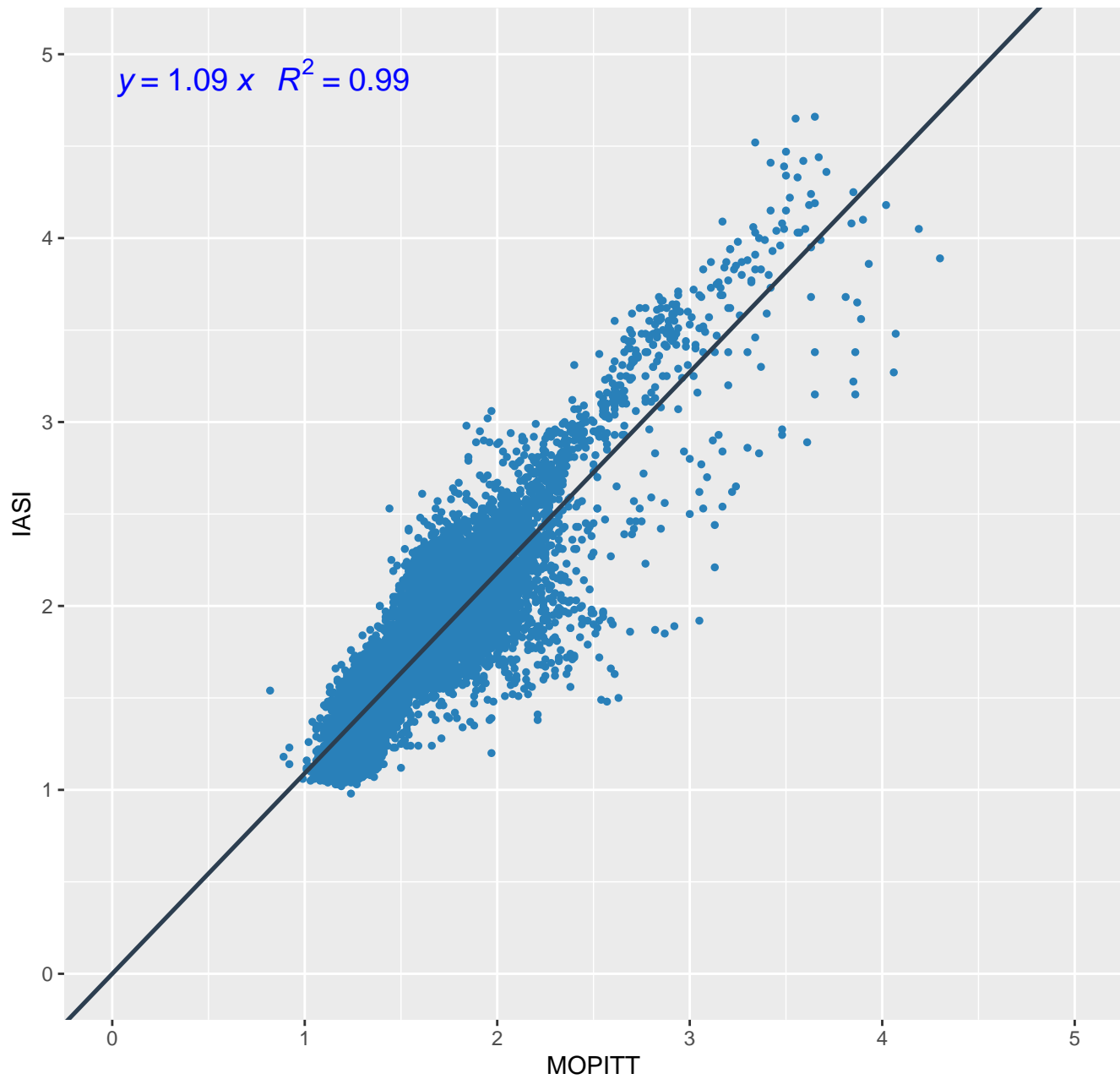
MOPITT IASI over water (Aug)
